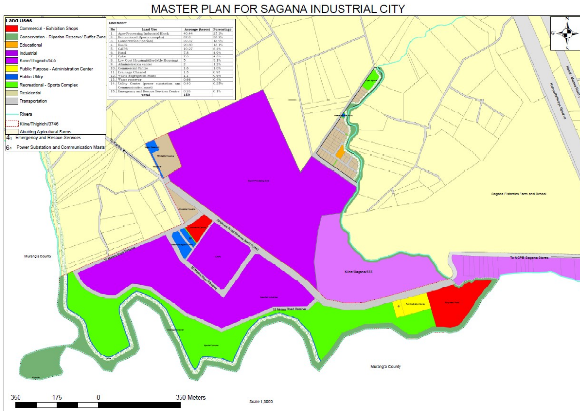
Figure 1: Master Plan for Sagana Industrial City
