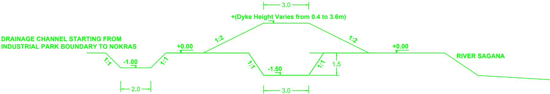
TYPICAL DYKE SECTION
